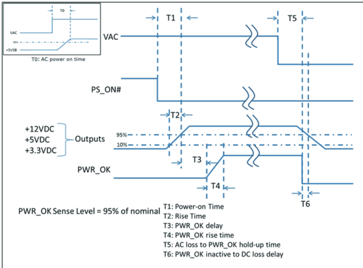
Figure 1 Time Diagram
